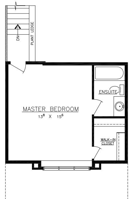
CAB-OVER AREA = 357 S.F.
